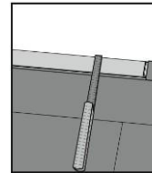
Fig 10. Last row (and first row). The minimum width of the last plank should be NOT LESS than 50 mm . Remember distance to wall is 12-15 mm. Tip! Put a spacer before measuring. Cut the planks lengthwise and glue the short ends. See instructions below.
